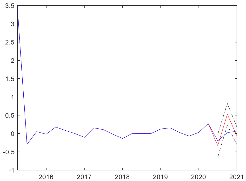
Figure 10: Forecasting - out of sample test of Tangerang total throughput
